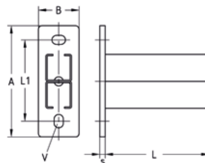
Profile 38/80
